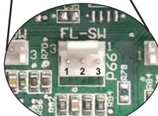
PSI/FLOW SWITCH CONNECTION
